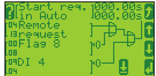
Figure 6-1: Display screen - Start req in AUTO
