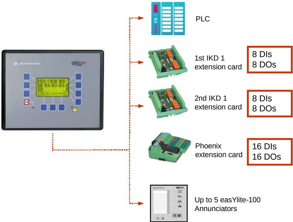
Figure 5-2: CANopen interface - external devices
