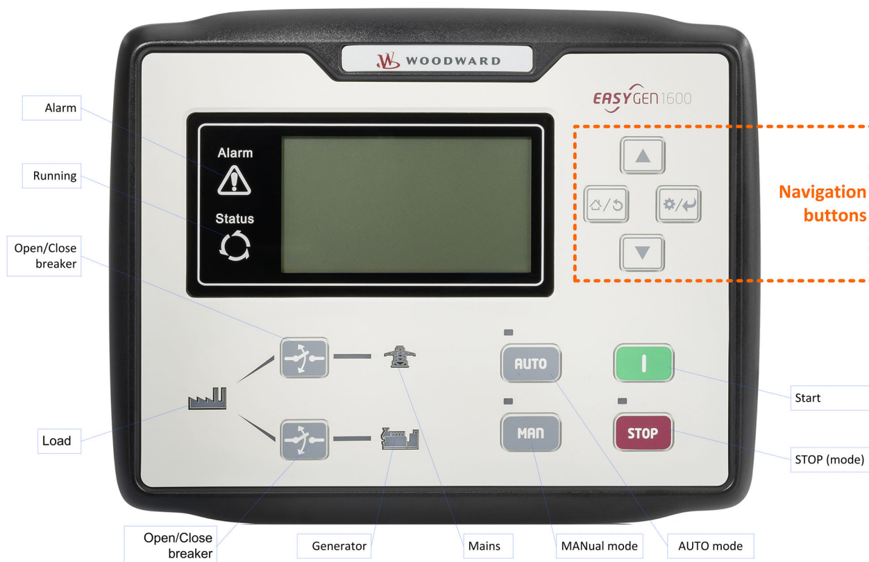
Rys. 2: HMI (tablica) easYgen-1600
