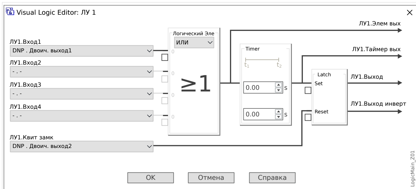
Рис. 40: Setting example from Smart view, to make a steady state signal from a DNP output signal.
